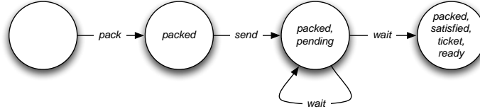
Figure 2.4: an expansion of \pi from example 2.3.1
